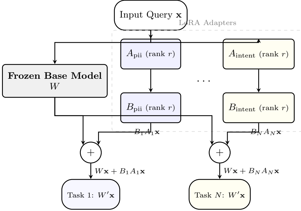
Figure 17: LoRA-based MoM inference architecture. The input query \mathbf{x} is processed by a single frozen base model ( W ). Each task-specific LoRA adapter pair ( A_i, B_i ) computes a low-rank perturbation B_i A_i \mathbf{x} . The base output and adapter perturbation are summed to produce task-specific classifications, enabling multi-task support with minimal memory overhead.
