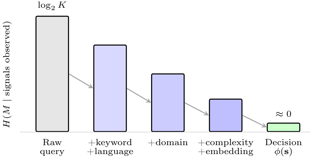
Figure 2: Entropy collapse during signal extraction (illustrative). Each additional signal reduces the routing uncertainty H(M \mid \cdot) from the uniform prior \log_2 K bits until the decision formula \phi(\mathbf{s}) yields a near-deterministic model selection. Bar heights are schematic rather than empirical measurements.
