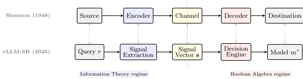
Figure 1: Structural correspondence between Shannon’s communication system ? and VSR’s routing pipeline. The dotted line marks the boundary between the information-theoretic regime (signal extraction maximizes mutual information with the routing outcome) and the Boolean-algebraic regime (the decision engine synthesizes routing policies from signal conditions via \{\wedge, \vee, \neg\} ?).
